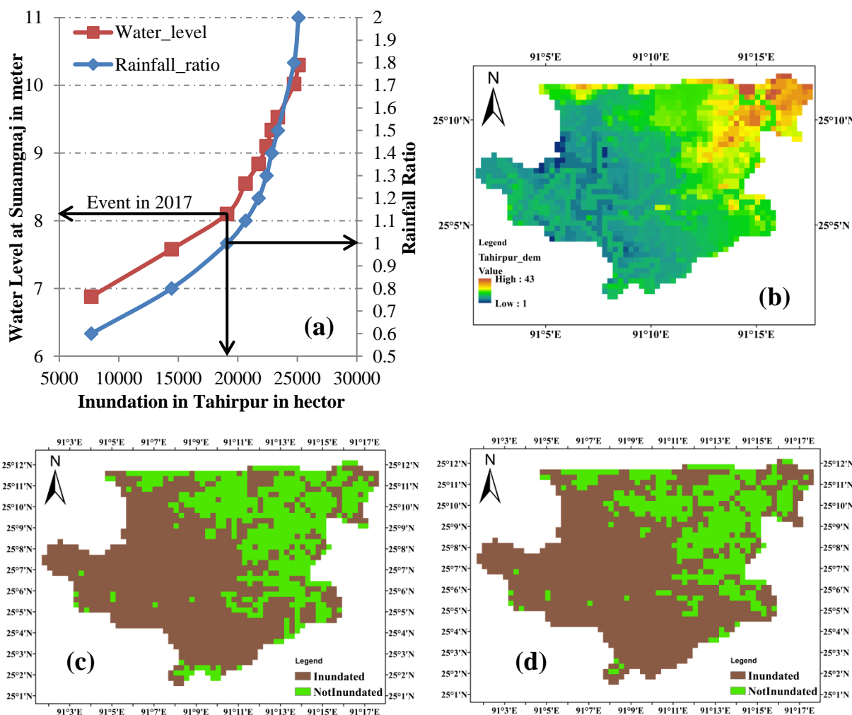
Figure 6: Tahirpur Upazilla (a) Relationship between Inundated Area due to Normalized Rainfall and Simulated Water Level at Sunamganj (b) Land Elevation (c) Inundation due to 10% increase in Rainfall (d) Inundation due to 30% increase in Rainfall
