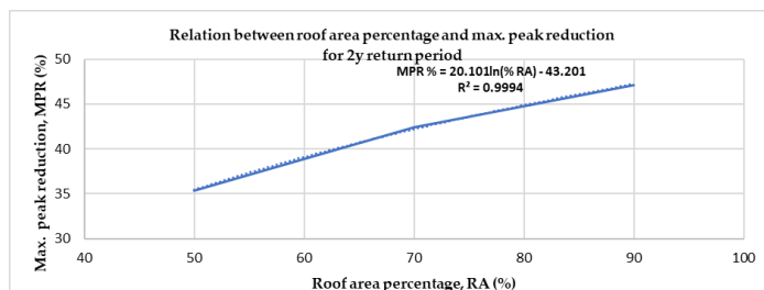
Figure 14: The relation between roof area percentage and maximum peak reduction for 2yr return period.
